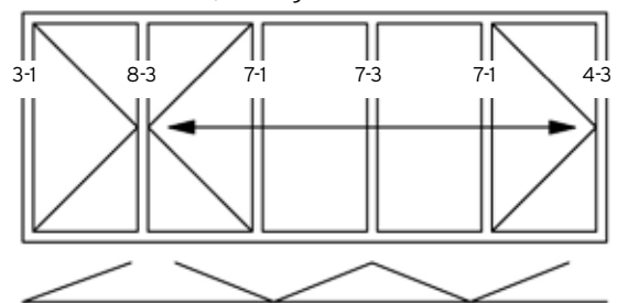
A - 1L 4LR Dreh / Swing
