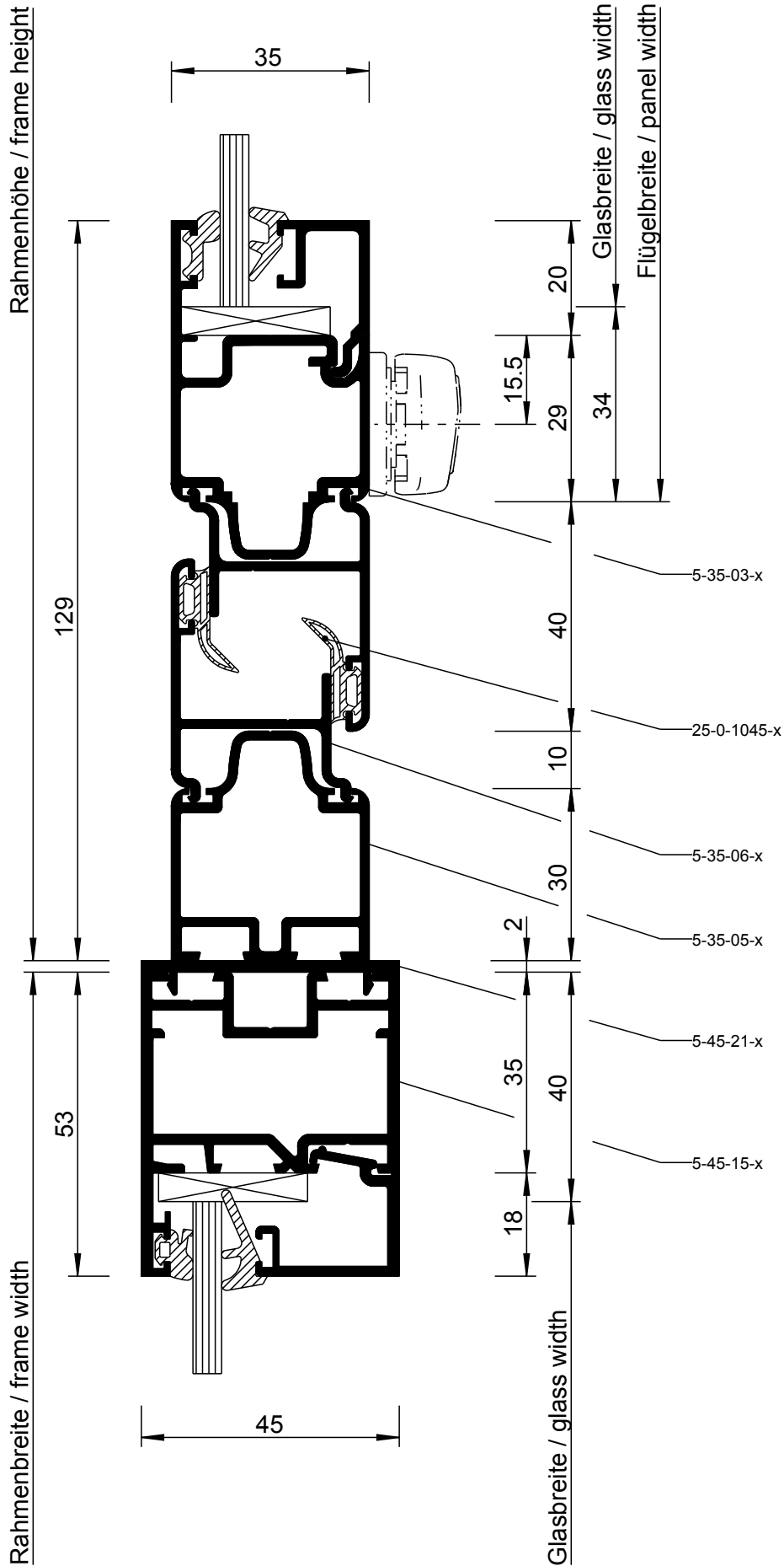
Detail 35-32-0
